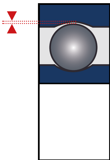
Radial Clearance Holgura radial
